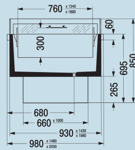
Visor ..35; Visor ..45
