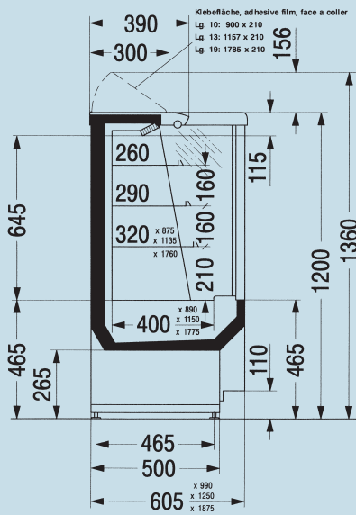
Presenter with level shelves, adjustable for height and slope
