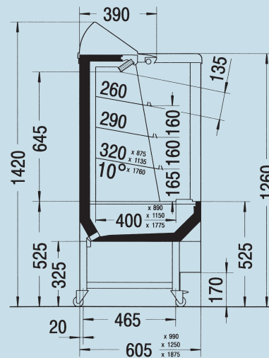
Presenter with 10° sloping shelves and caster base
