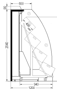
Monaxis 80-NCH.B2 with trolleys, height 2040 mm
