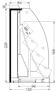
Monaxis 80-NCH.B2L with trolleys, height 2220 mm
