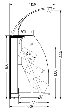
Mirado 60-NCH with trolleys and external lighting
