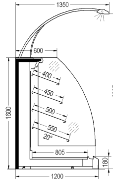
Mirado 82-NC with slim-line display shelves and external
