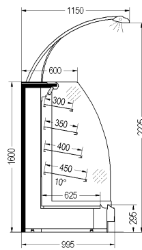
Mirado 63-NC with slim-line display shelves and external
