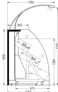
Mirado 80-NCH with trolleys and external lighting
