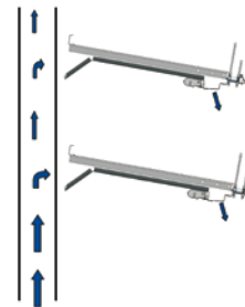
Air flow through hollow chambers in the shelves Monaxis SL
