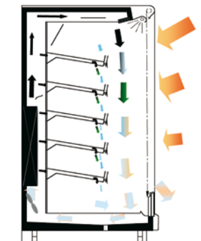
Functional diagram for the sequential air curtain Monaxis SL
