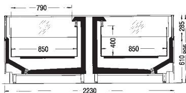
Ivando SG3.B4/B8
