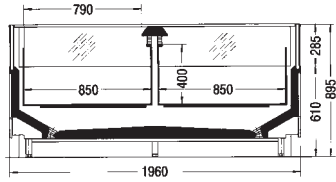
Irios SG3.B4/B8
