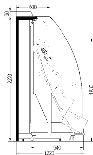
Monaxis 80-NCH.B2L with trolleys, height 2220 mm
