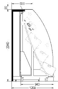
Monaxis 80-NCH.B2 with trolleys, height 2040 mm
