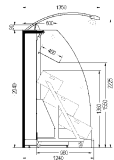
Monaxis 80-NCH with 1 row of display shelves and trolleys
