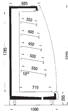
Marena 73.A4 L
