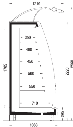
Marena 73.A3 L with external lighting (optional)
